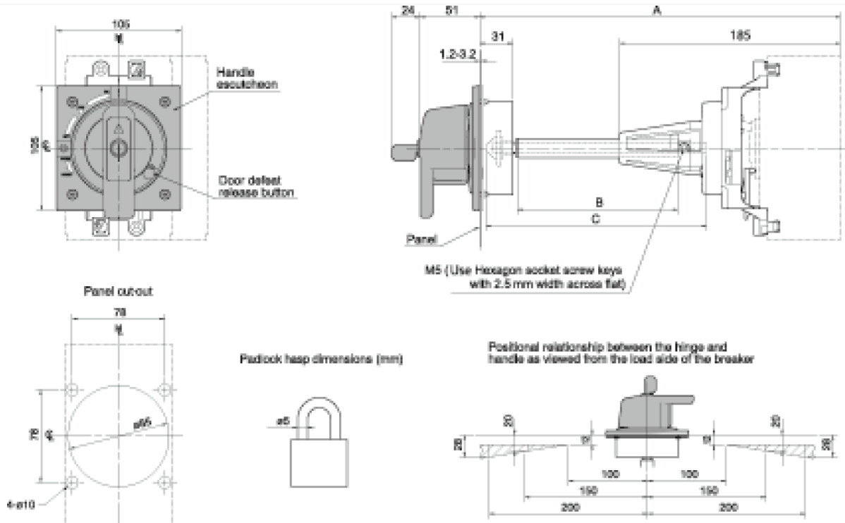
Dimension Diagram
