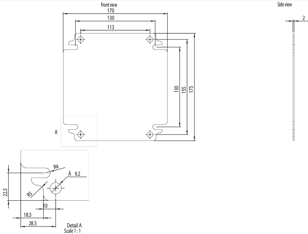
Dimension Diagram
